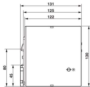
Dimensional drawing
